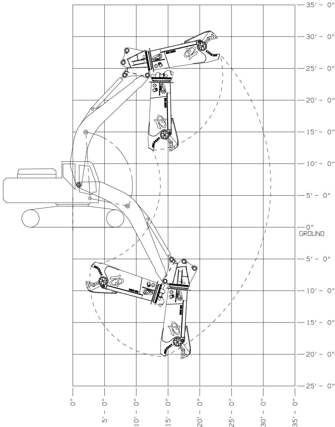
SN622160 ON A KOBELCO SK300LC-10 (MSD 2250R W/ 221140 DUAL MULTI HEAD)
