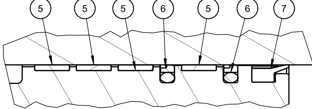
DETAIL B (1 : 1)
