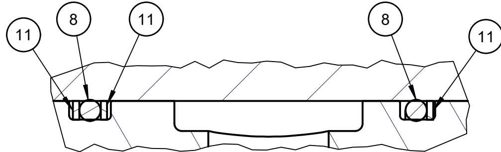
DETAIL E (1 : 1)
