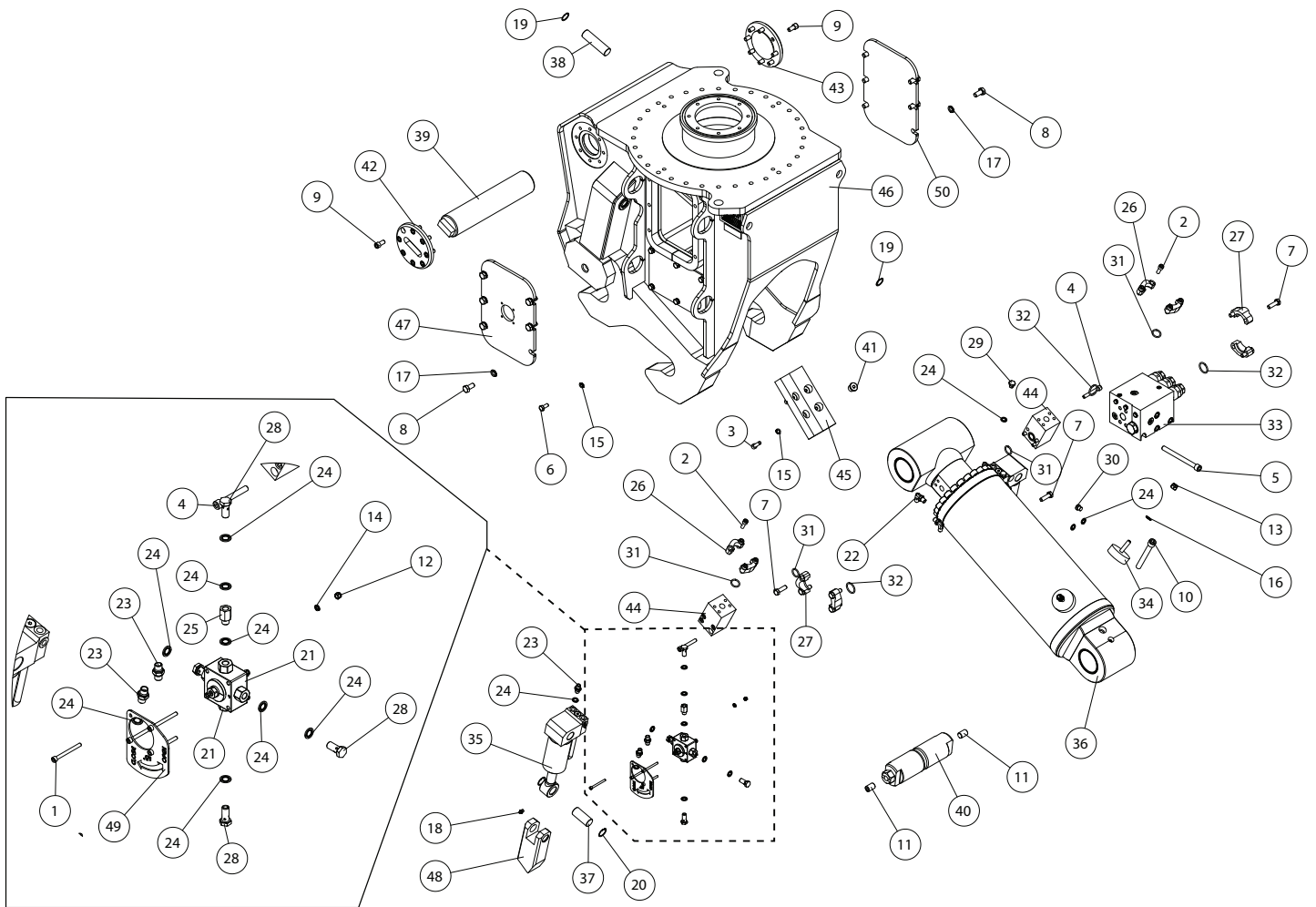
MRX180 Body Parts Illustration
