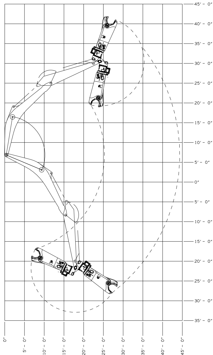
LABOUNTY MSD 1500R - 3RD MEMBER BOLT ON HEAD KOBELCO SK350LC-10 W/ 6.50M BOOM, 4.15M STICK APPROXIMATE RANGE
