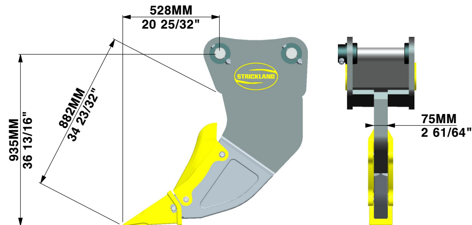
REPLACEABLE RIPPER SHROUD (GG-GET013370031-0)
